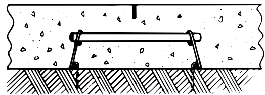
CONTRACTION (sawed joint)
